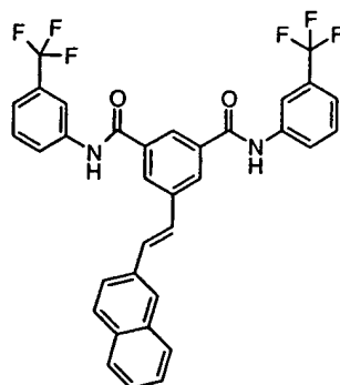
Compound # 26
